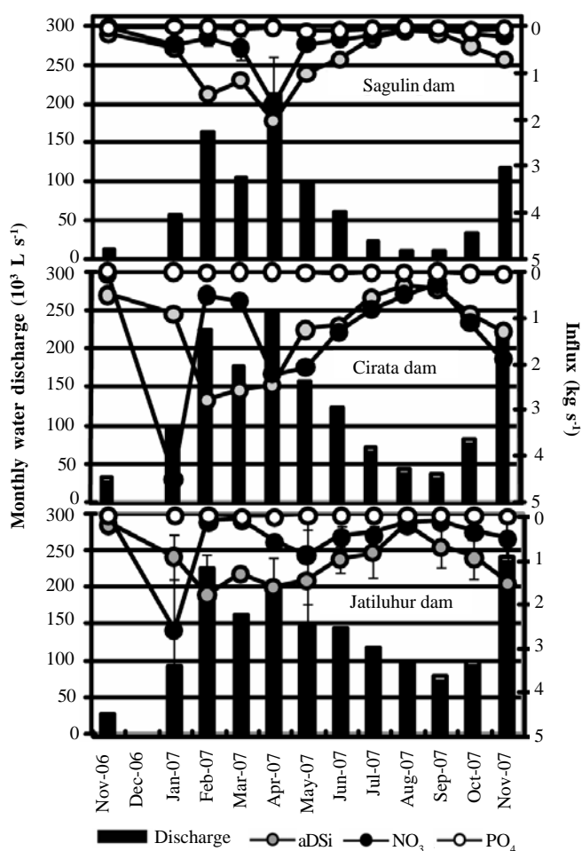
Figure 4. Monthly mean influx of DSi, NO 3 and PO 4 (kg s -1 ) in Saguling, Cirata and Jatiluhur dams.
